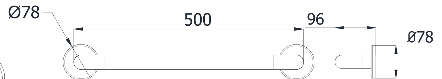
VISTA FRONTAL
