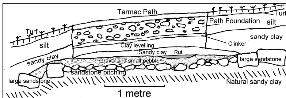
Buried road at Duffield Bank House. After Cobbold and Thorpe, 2017. (W-E)
