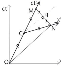
Figure 2. Two inertial frames are represented in two dimensions, R(O; ct, x) , and R'(C; ct', x') . The latter is constructed with respect to the first using Einstein synchronization rule. ON and NM together represent the trajectory of a light beam emitted from O in the direction of x increasing, and bouncing back in N . C is the middle of OM . The x' axis is supported by CN following the synchronisation rule. H is the middle of MN . A simple geometry reasoning in two dimension shows that x' is the symmetric of ct' through the orthogonal symmetry with respect to CN , which is parallel to ON .
