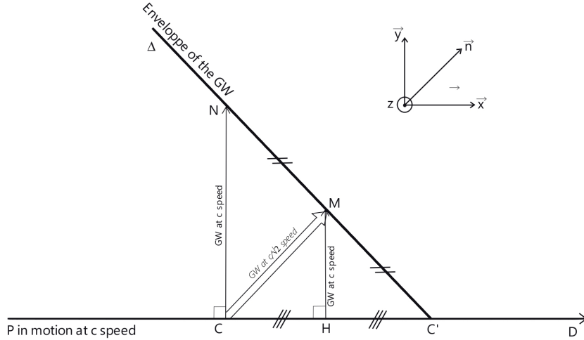
Figure 1. The GW generated by a P uniformly moving relativistic particle is shown in two space dimensions. D is the trajectory of P . The space-time deformation generated by P propagates perpendicularly to D from C to N at the c speed, and also from H to M at the c speed. H is the middle of CC' and M is the middle of NC' . \Delta is the envelope of the GW. This envelope propagates at the c/\sqrt{2} speed from C to M .
