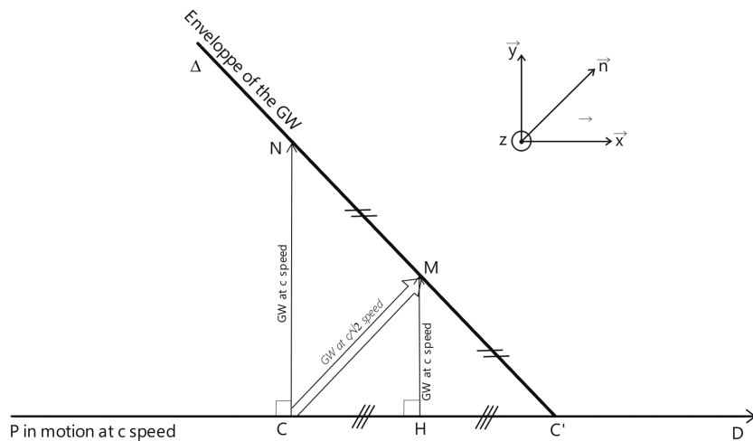
Fig. 1. The GW generated by a P particle moving at the speed of light is shown in two space dimensions. D is the trajectory of P . The space-time deformation generated by P propagates perpendicularly to D from C to N at the c speed, and also from H to M at the c speed. H is the middle of CC' and M is the middle of NC' . \Delta is the envelope of the GW. This envelope propagates at the c/\sqrt{2} speed from C to M .
