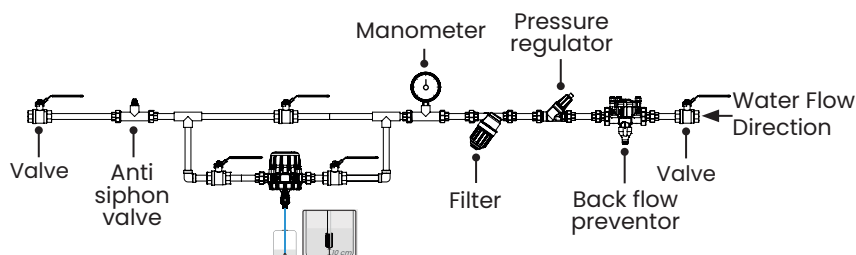
Fig. 2 - Installation illustration
