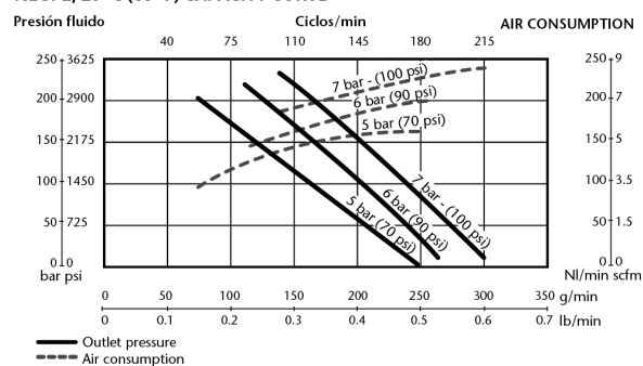
NLGI-2, 20 °C (68 °F) CAPACITY CURVE
