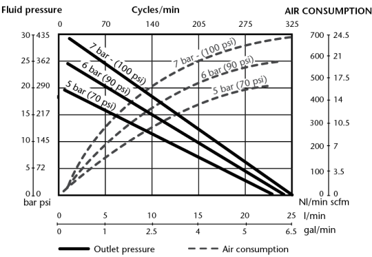
SAE 30, 23 °C (73 °F) CAPACITY CURVE
