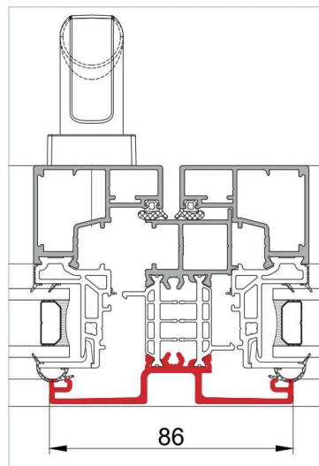
Battue standard
