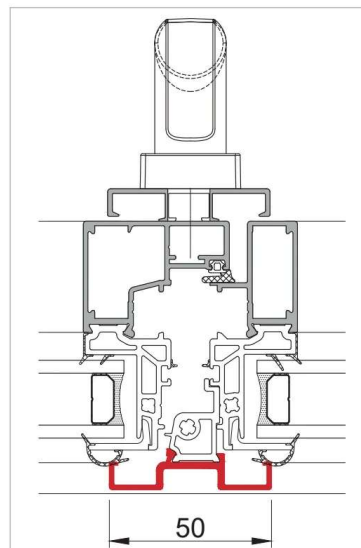
Battue mince (option)
