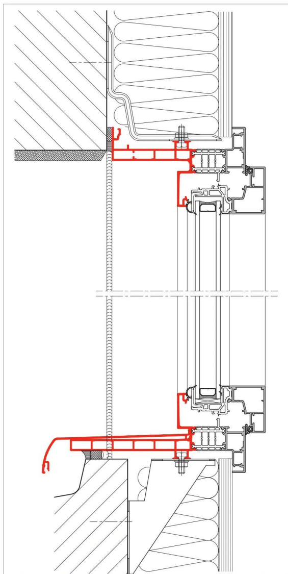
Coupe technique verticale
