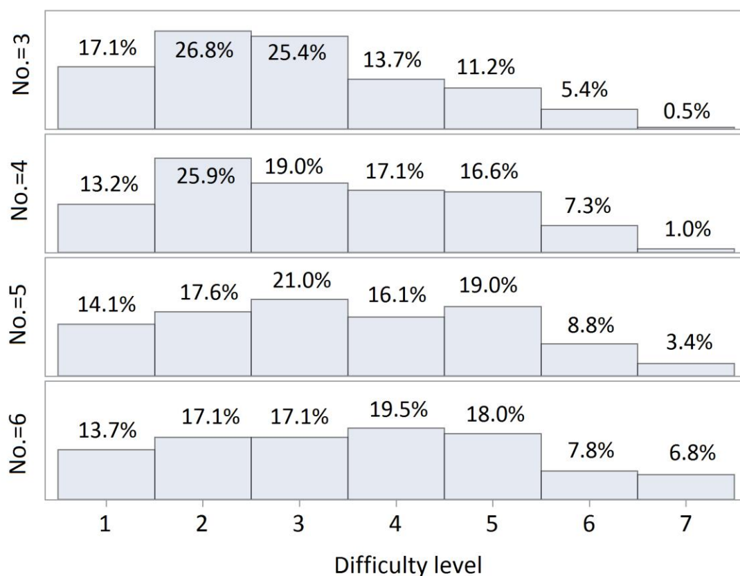
Figure 4-5. Difficulty level rating histograms
