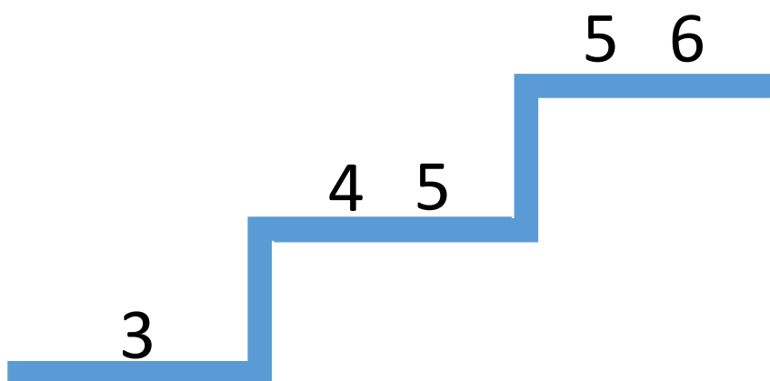
Figure 4-8. Summary plot of effort level ratings comparisons
