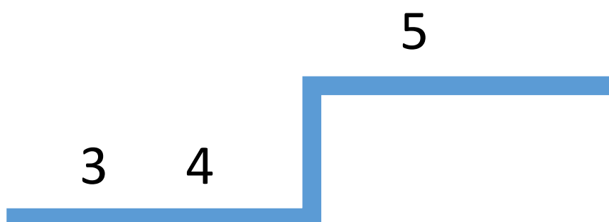
Figure 4-10. Summary plot of survey duration comparisons
