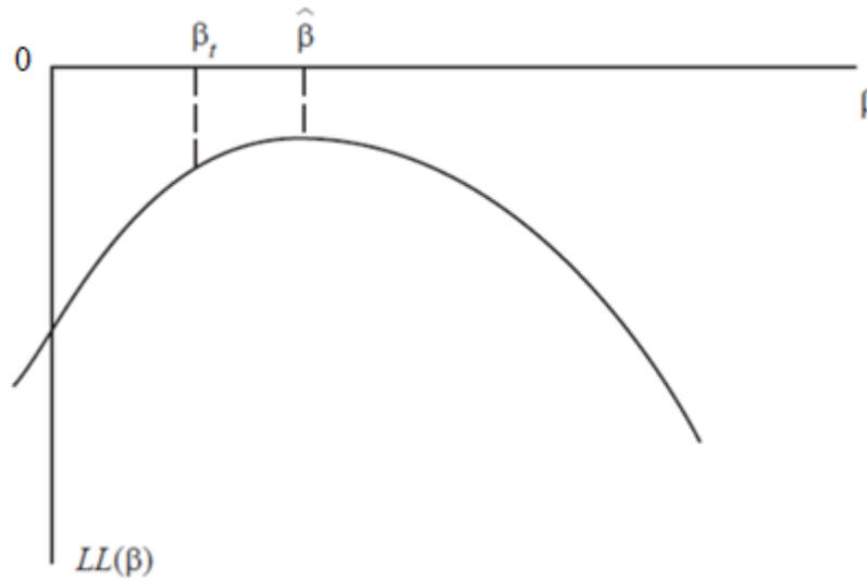
Figure 6-3. Maximum likelihood estimate (Train, 2002)
