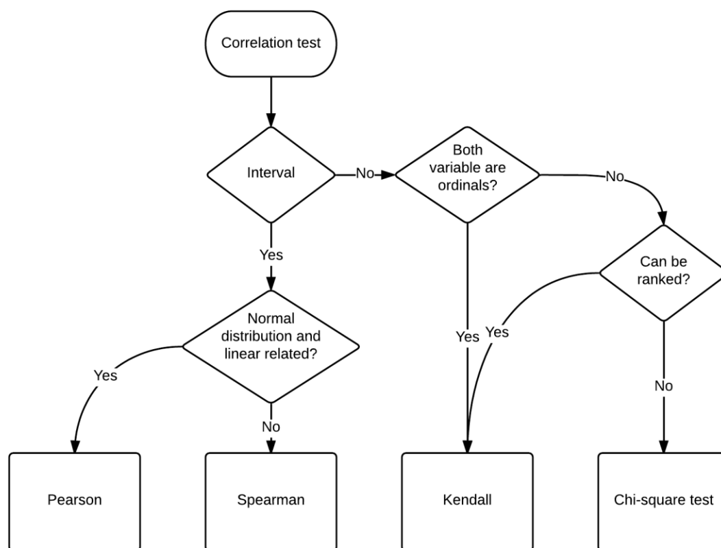
Figure 4-1. Flowchart of correlation test approach
