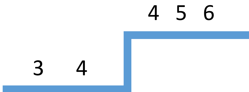
Figure 4-9. Summary plot of difficulty level ratings comparisons
