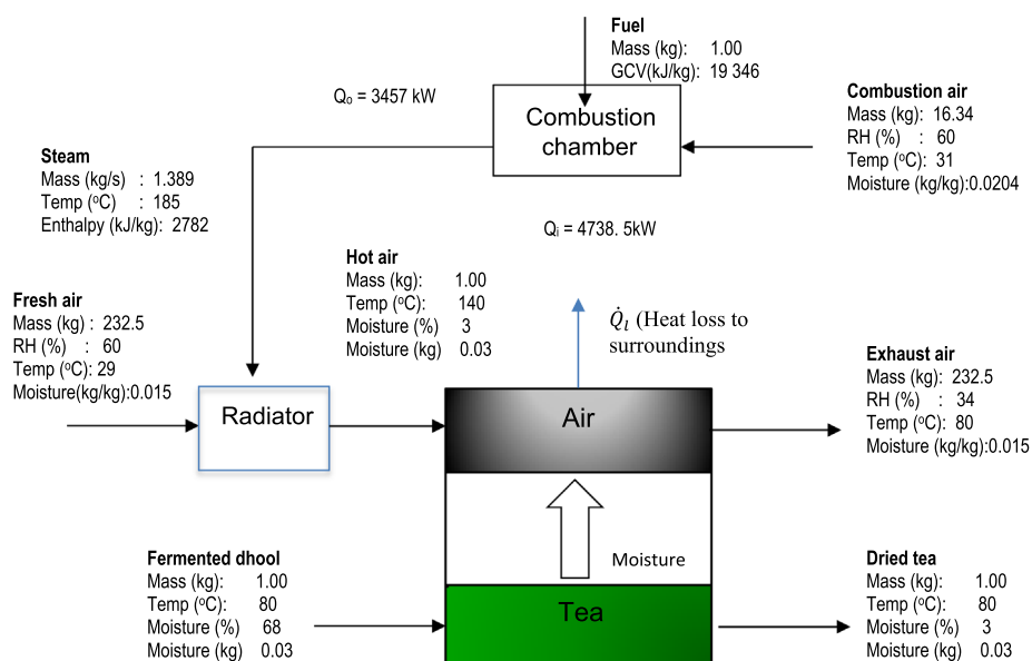
Fig. 5. Energy calculations for drying tea leaves.
