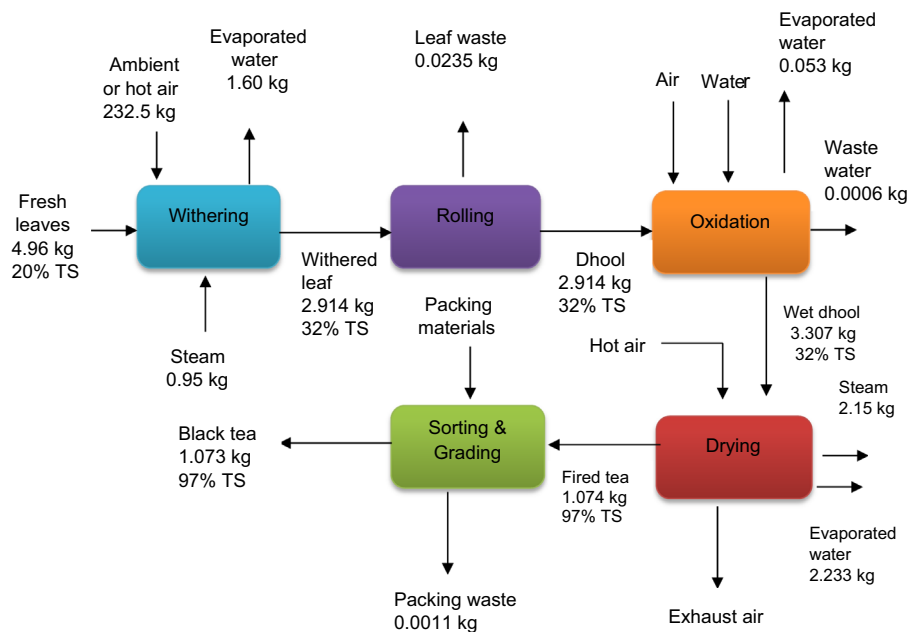
Fig. 3. Material balances in black tea processing factory.
