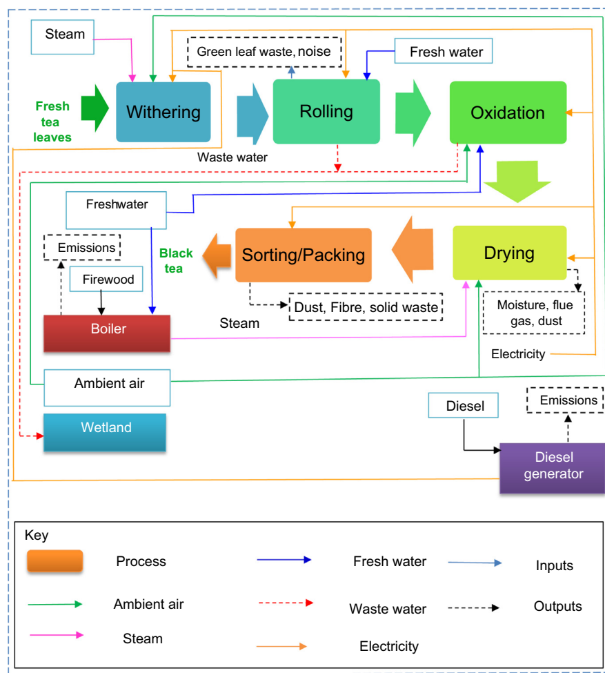
Fig. 1. Process flow diagram for tea factory.
