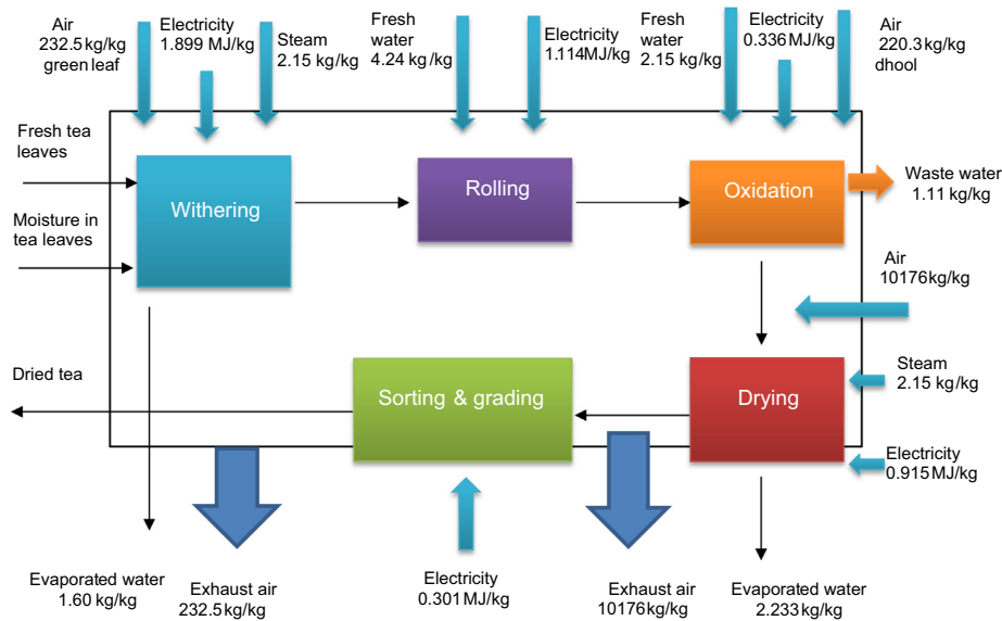
Fig. 4. Energy flow diagram of tea processing factory.
