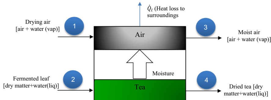
Fig. 2. Schematic of drying process with inputs and outputs [28].
