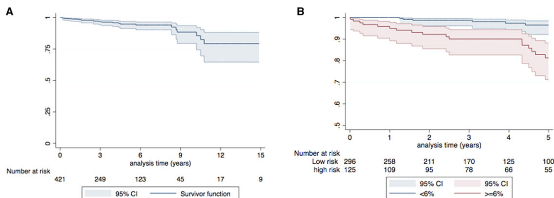
Figure 2 Kaplan–Meier curves showing event-free survival (A) for whole cohort (B) by risk category ‘high risk’ (hypertrophic cardiomyopathy Risk-Kids estimated 5-year risk \geq 6\% ) and ‘low risk’ (hypertrophic cardiomyopathy Risk-Kids estimated 5-year risk < 6\% ) [hazard ratio of 6.16 (95% confidence interval 2.43–15.65), P < 0.001 ]. CI, confidence interval.
