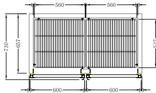
PLAN (顶视)
