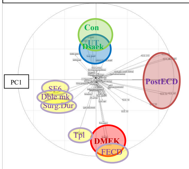
C. Third PCA: ECD not reweighted
