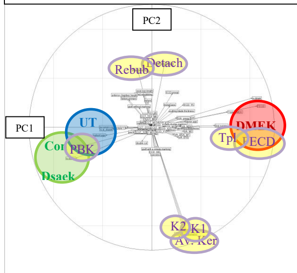
A. First PCA: VA, ECD, CGT, & CCT all reweighted to 1
