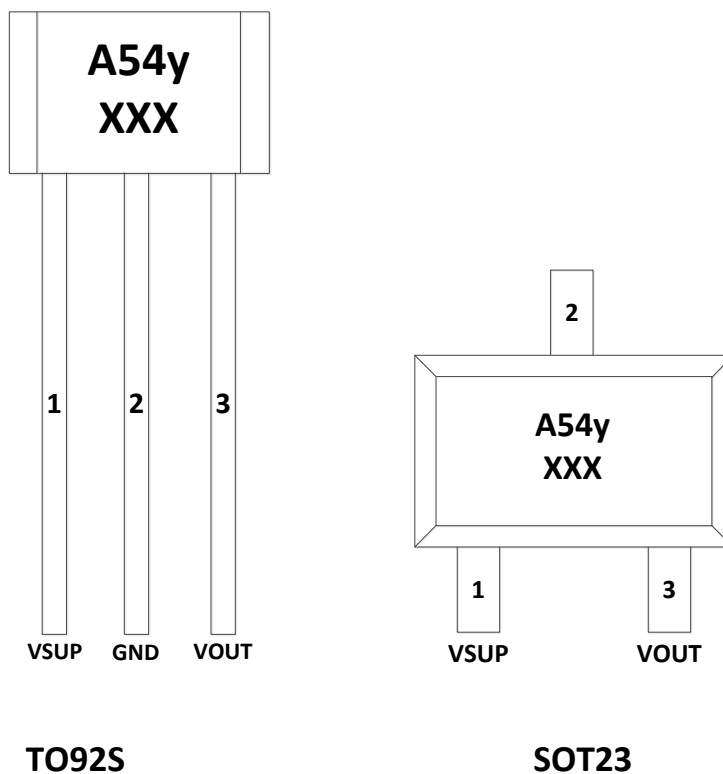
Fig.4: Pin assignment of TO92S and SOT23
