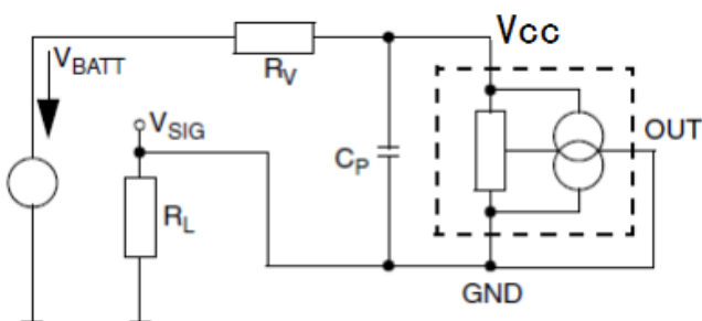
Fig. 6: Example 2-wire application circuit 2
