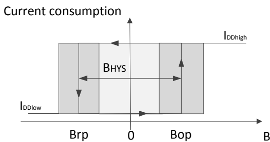
Fig. 1: Definition of magnetic switching points for 2-wire unipolar sensor.
