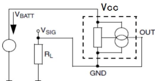
Fig. 5 : Example 2-wire application circuit 1
