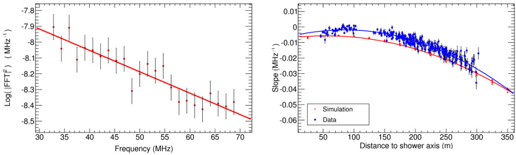
Figure 1. Left: distribution of \log_0 |\text{FFT}|^2 as function of frequency for one antenna of one selected event; the distribution has been fitted with a linear function, taking into account 20% uncertainty on the |\text{FFT}|^2 converted into logarithmic values. Right: distribution of the linear-fit slope as function of distance to the shower core for one selected event (blue squares) and the corresponding simulated event (red stars). Both distributions have been fitted with a parabolic function.
