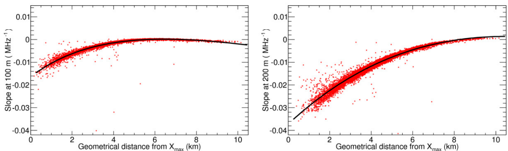
Figure 3. Distribution of the linear-fit slope (red stars) for simulated events as function of D_{\text{max}} at 100 m (left) and 200 m (right) from the shower axis. Both distributions have been fitted with a 4-parameters function: p_0 \cdot \exp(-p_1 \cdot D_{\text{max}}) + p_2 + p_3 \cdot D_{\text{max}} .
