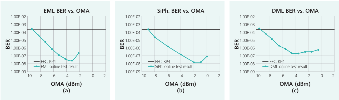
Figure 7 – (a) EML BER vs. OMA results based on commercial available 400G DSP ASICs; (b) Silicon Photonics BER vs. OMA results based on commercial available 400G DSP ASICs, (c) DML BER vs. OMA results based on commercial available 400G DSP ASICs
