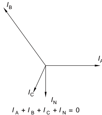
FIGURE 3 PHASOR DIAGRAM OF CURRENTS IN UNBALANCED THREE-PHASE CIRCUIT
