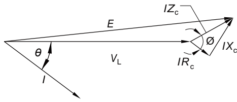
(a) \cos \theta = 0.8 lagging
