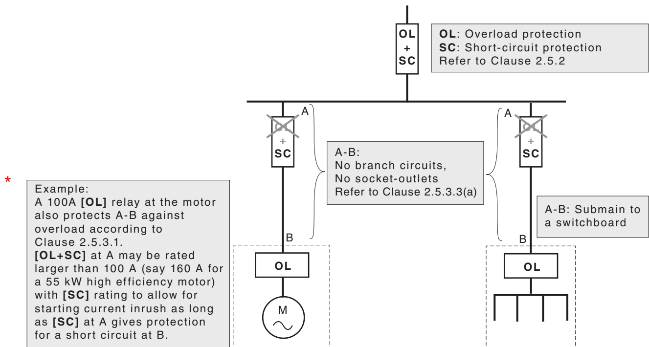
FIGURE 2.3 MANDATORY OMISSION OF OVERLOAD AND/OR SHORT-CIRCUIT PROTECTION
