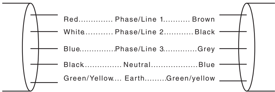
FIGURE 3.2 MULTIPHASE CABLES
