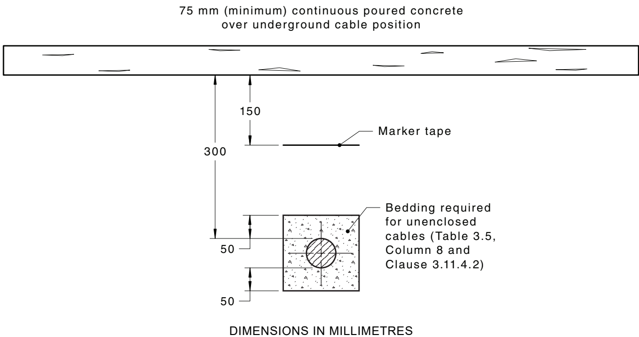
FIGURE 3.10 EXAMPLE OF A CATEGORY A WIRING SYSTEM WITH CABLE LOCATED BELOW POURED CONCRETE OF 75 mm MINIMUM THICKNESS
