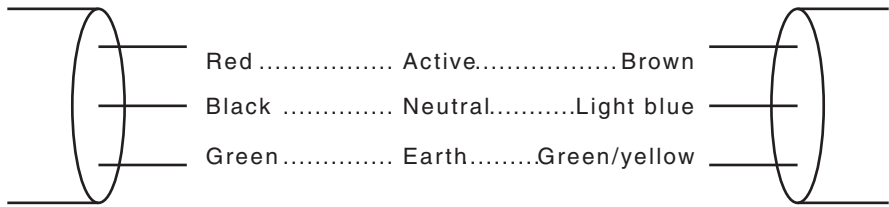
FIGURE 3.1 SINGLE-PHASE CABLES
