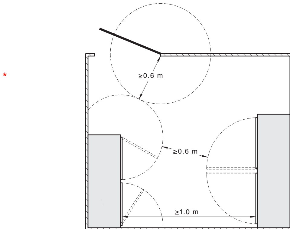
FIGURE 2.23 ACCESS TO SWITCHBOARDS—FACING SWITCHBOARDS
