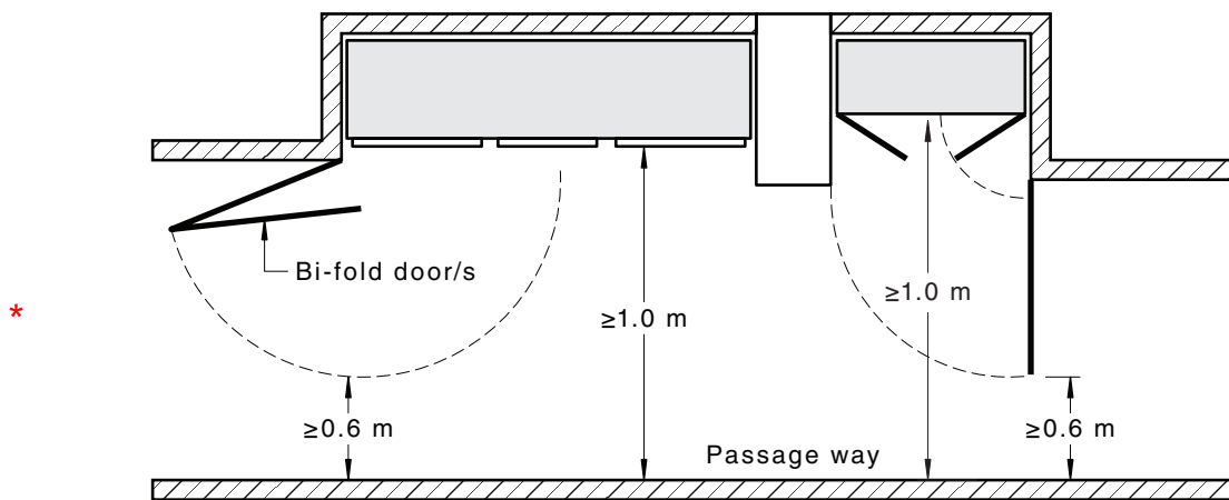
FIGURE 2.22 ACCESS TO SWITCHBOARDS—SWITCHBOARD DOORS THAT OPEN INTO ACCESS WAYS OR NARROW PASSAGE WAYS
