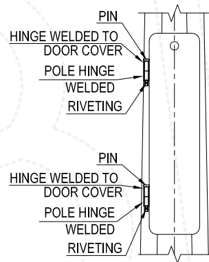
HINGE ARRANGEMENT DETAIL "Z"
