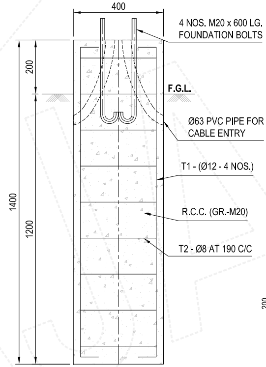
DETAIL OF CIVIL FOUNDATION
