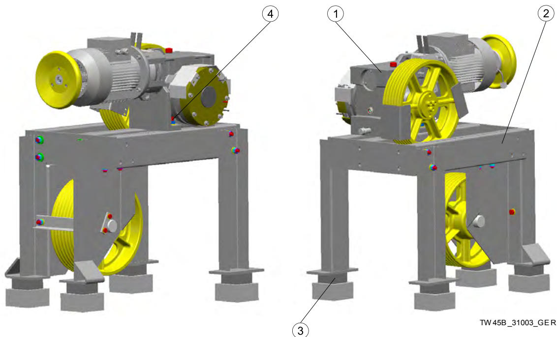
Fig. 3-8: TW45B M SR machine base frame (shown: machine base frame in right-hand configuration of the rope pulley with machine in horizontal motor position and traction sheave position on left, incl. emergency brake - NBS)
