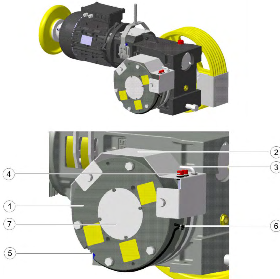
Fig. 2-3: TW45C machine - version for location in machine room / with emergency brake, NBS (shown: horizontal motor position, traction sheave position–on left)
