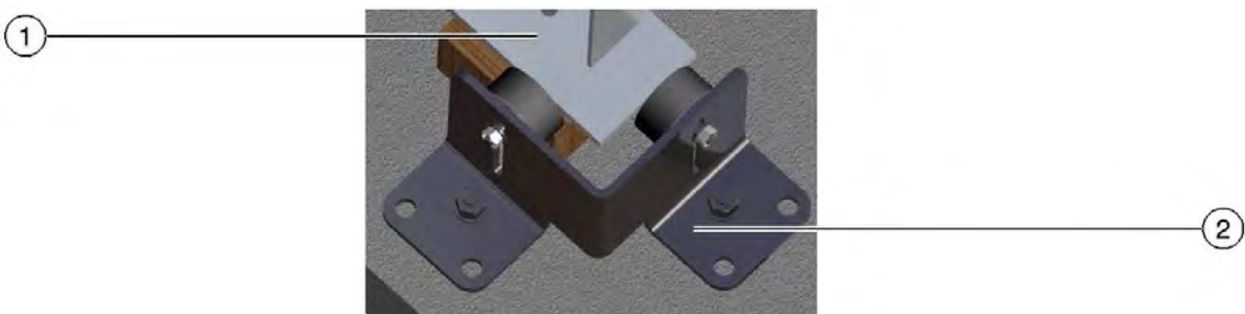
Fig. 3-12: Earthquake safeguard complying with EN81-77 on machine base frame (shown is the shift protection)
