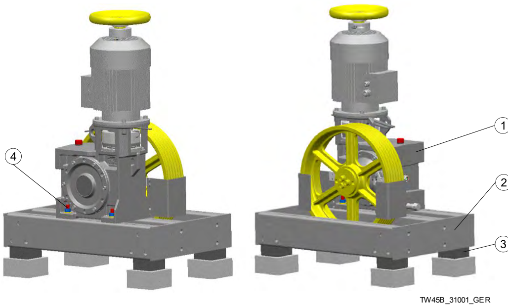
Fig. 3-7: TW45B O SR machine base frame (shown with machine in vertical motor position and traction sheave position on left)
