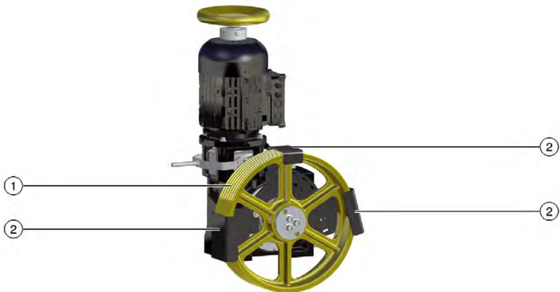
Fig. 2-5: TW45C machine - version for location in machine room (shown: traction sheave position on left / motor position vertical and earthquake safeguard complying with EN81-77)
