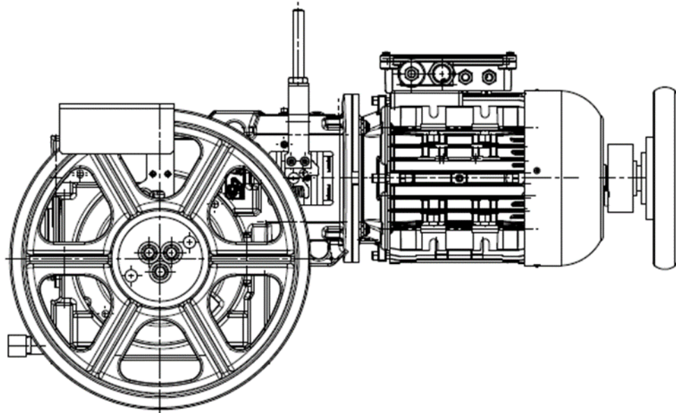
Fig. 3-6: Machine TW45C - Version for installation site - machine room with rope outlet direction - horizontal (shown version with traction sheave position - left and motor position - horizontal)
