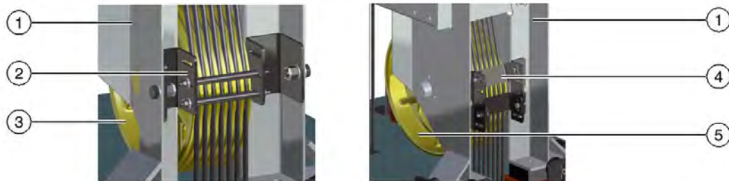
Fig. 3-11: Safeguard measures on AY machine frame unit in accordance with EN 81-77
