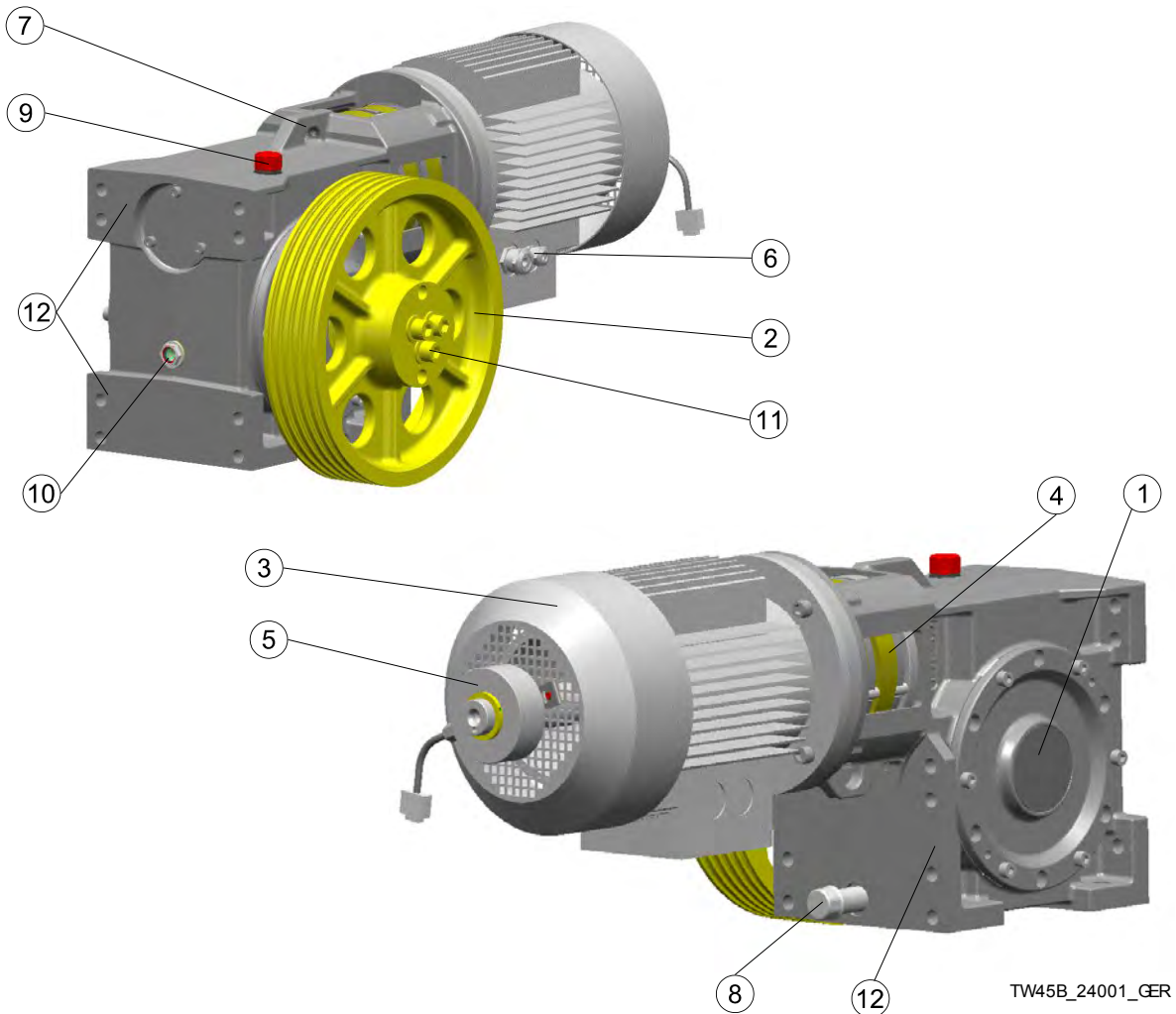
Fig. 2-6: TW45C machine - version for location in headroom (shown: version with traction sheave position on left)
