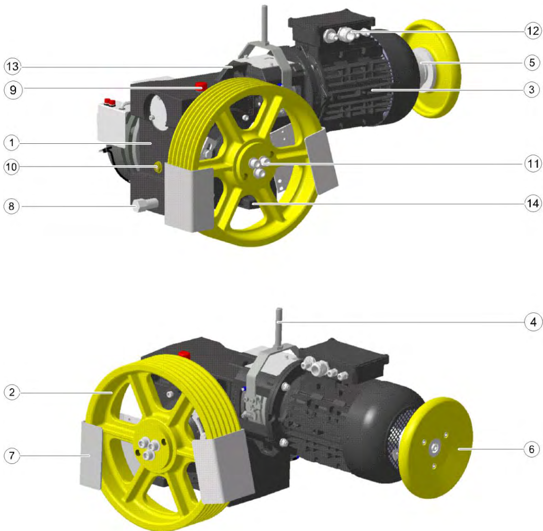
Fig. 2-2: TW45C machine - version for location machine room / motor position horizontal IMB5 (shown with traction sheave position left, with emergency brake system)
