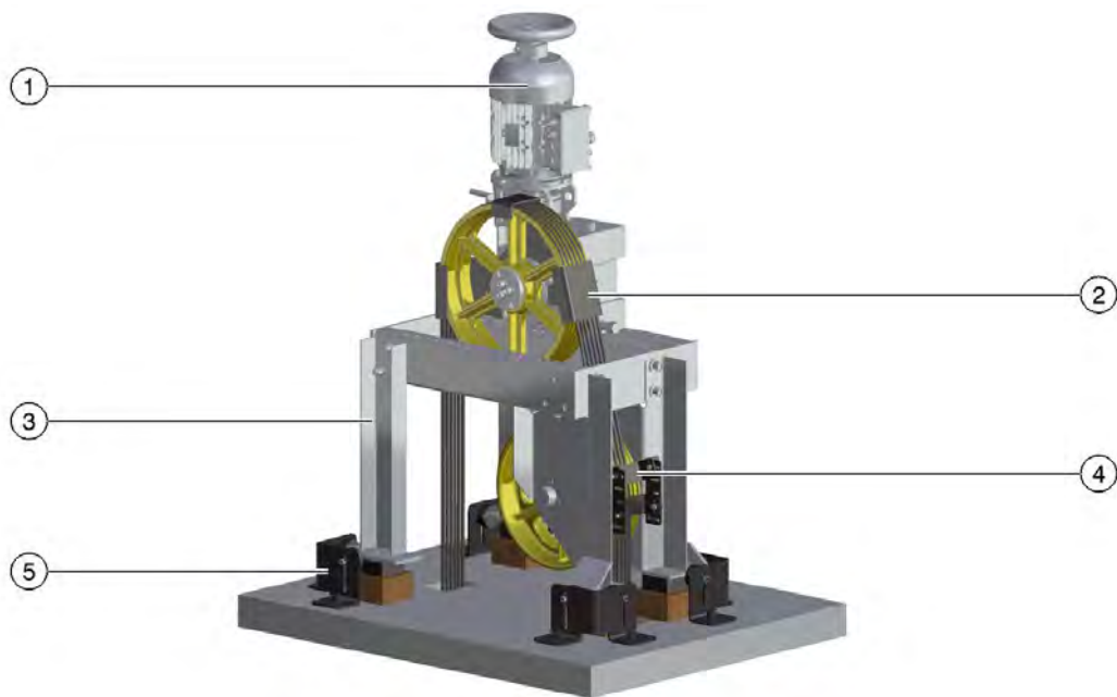
Fig. 3-10: Safeguard measures on AY machine frame unit in accordance with EN 81-77
