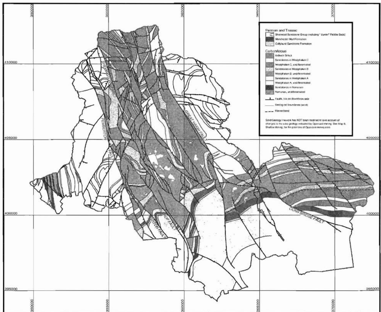
Figure 2 Simplified bedrock geology (reduction of Map 2).
