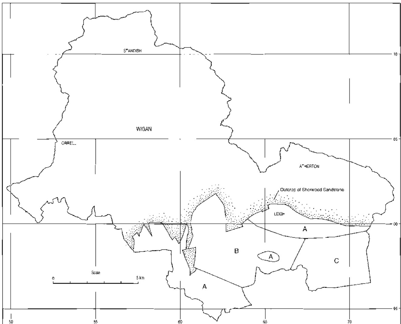
Figure 20 Zones of different groundwater chemistry in the Permo-Triassic aquifer south of Wigan.
