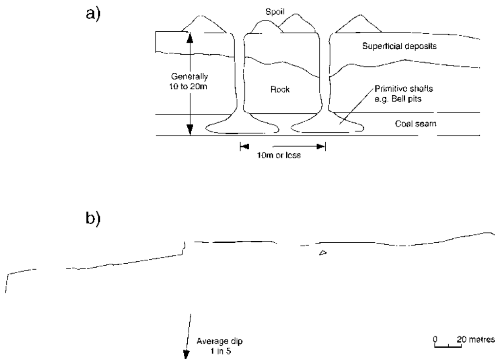
Figure 22 Diagrammatic cross section of bell pits found in opencast sites.
