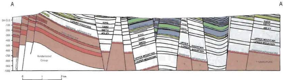
Figure 6 Graben structure in the bedrock below the Wigan area.
