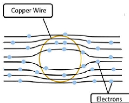
Figure 53: Represents the exothermic equation, the force in is greater than the force out , this is the electric field current invading the positive atom ions causing frictional force, this occurs after the Newman Point .
