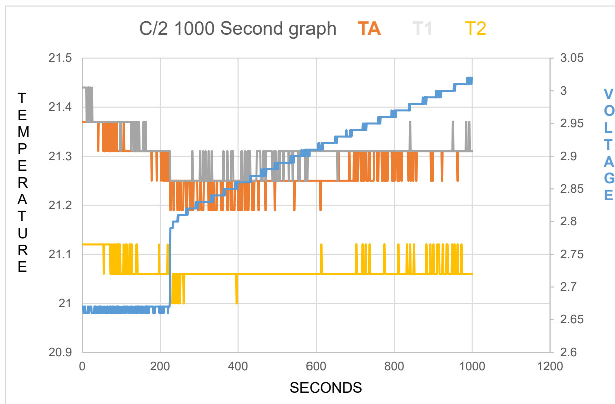
Figure 36: TA shows Endothermic cooling reaction for 7 mins 34 seconds at start of electric field charge when EMF is applied.
