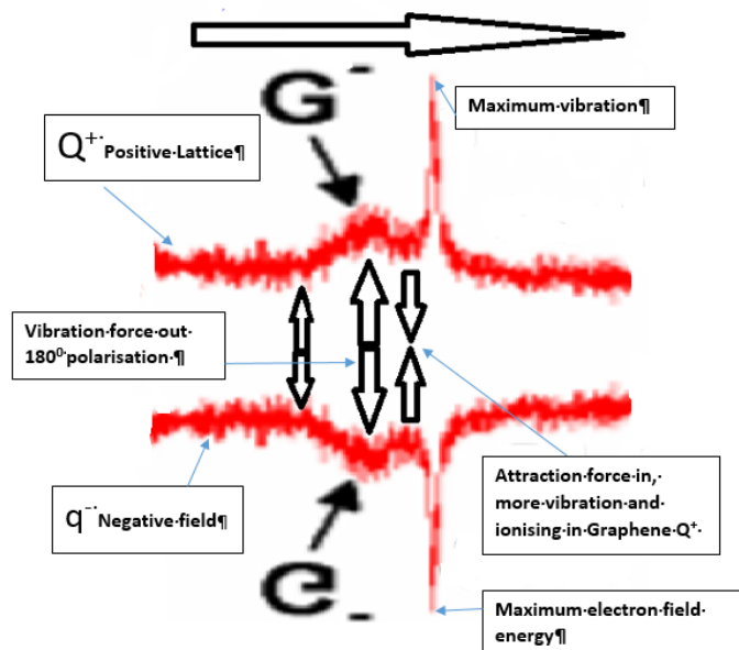
Fig y: Electric field depiction from Raman Shift Data: We know the sample is in an electric field state due to power to the LED as shown in Fig 4b of [105].
