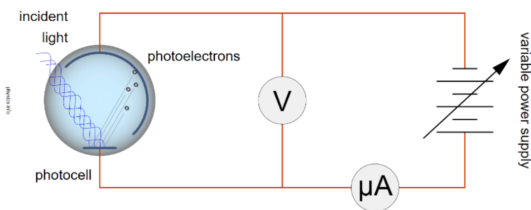
Figure 15: Experiment devised by Philipp Lenard, Nobel prize winner 1905. Schematic of experiment to show and measure the photoelectric effect.
