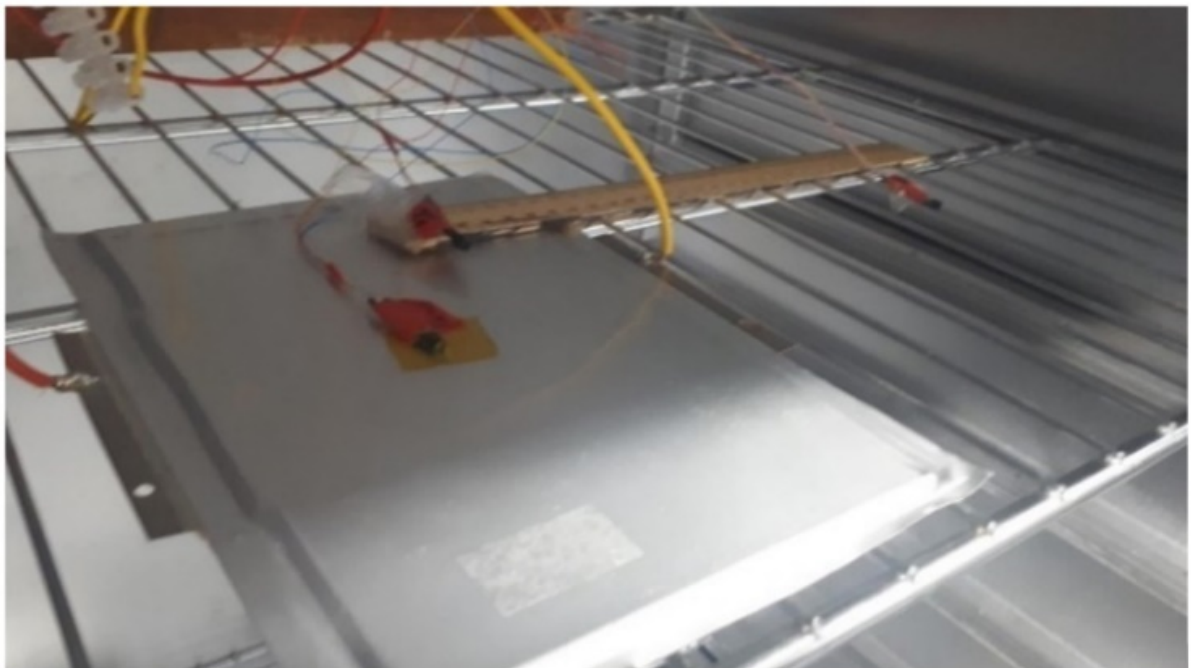
Figure 34: Lithium battery with temperature sensors,
