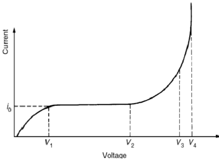
Figure 19: Kuffel graph: Townsend's current-voltage relationship in pre spark region.
