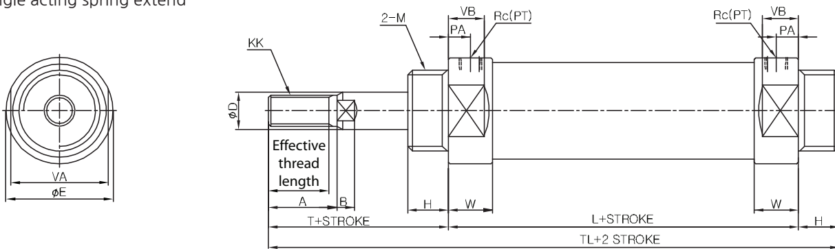
Single acting spring extend
