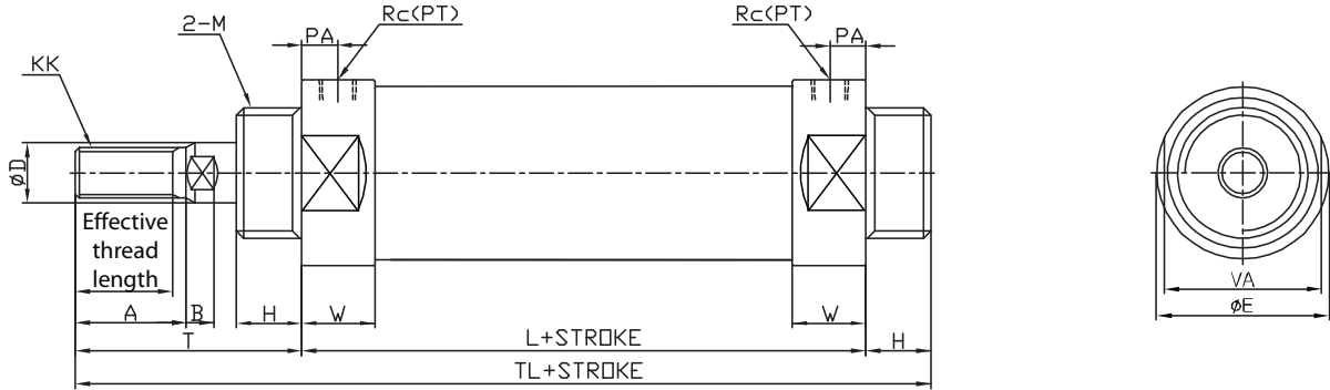
Single acting spring return
