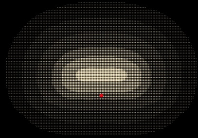
TS11 Asymmetric Side and Forward Throw
