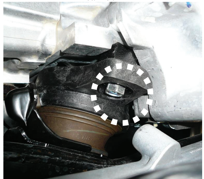
Rear Bolt
