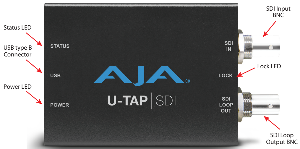
Figure 4. U-TAP-SDI Connectors and LEDs (on Each Side)
