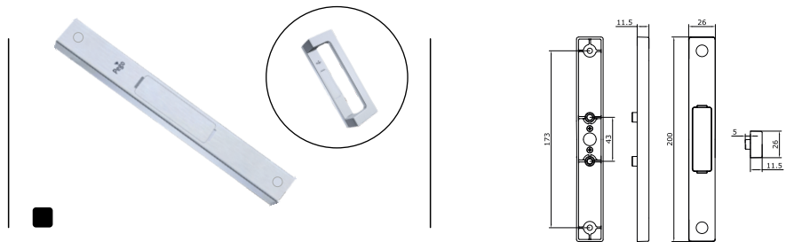
SLIDING DUMMY LEVER METRO HANDLE
