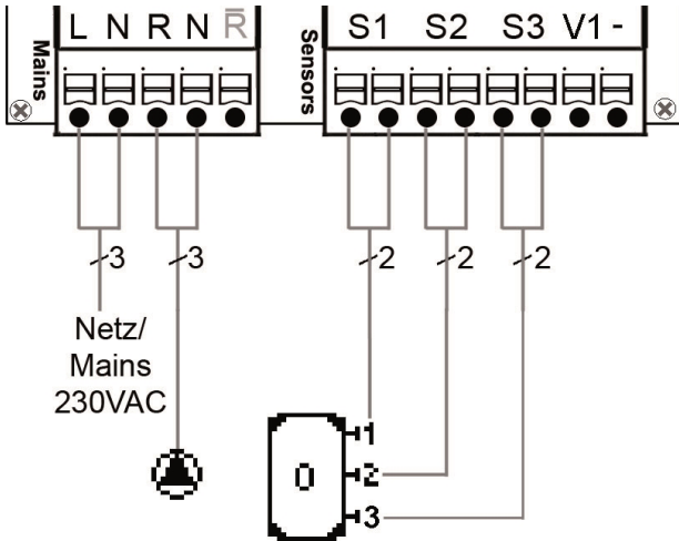
Programm 6 Thermostat
