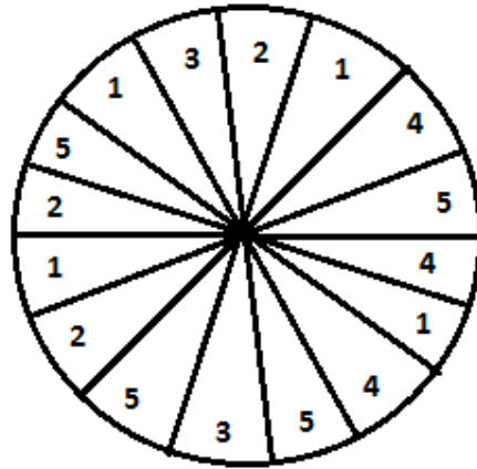
Probability - Spinner
