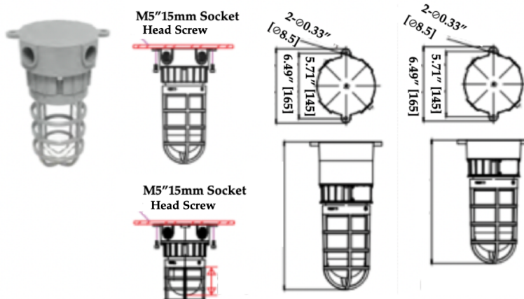
Option 1: Ceiling Mounting
