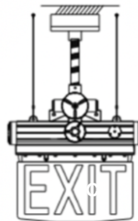
Option 3: Pendant Mounting With Safe Wires
