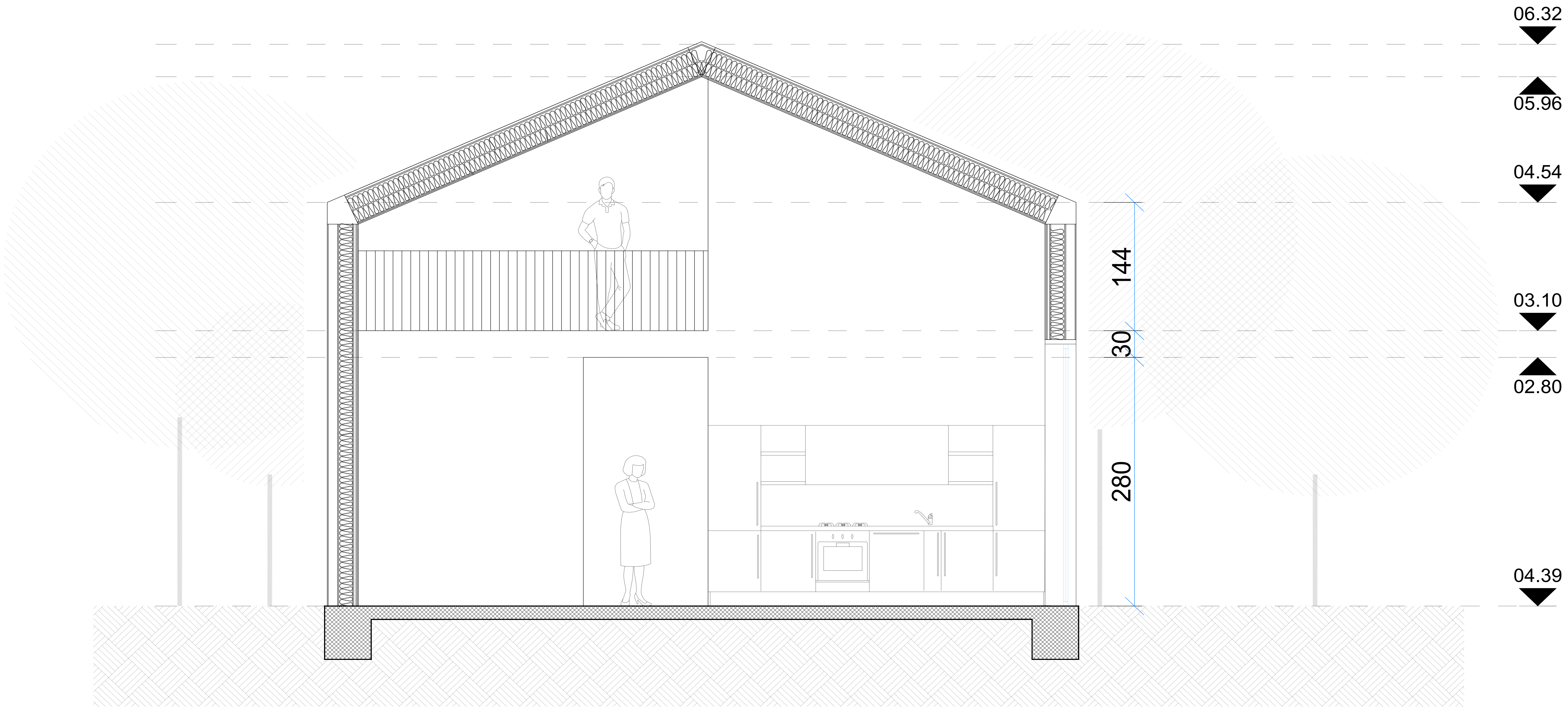
A- Section
