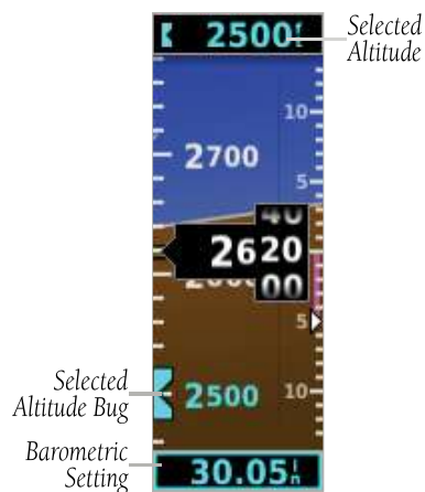
Figure 2-9 Altimeter
