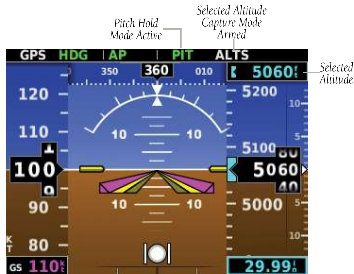
Figure 3-8 Pitch Hold &amp; Selected Altitude Capture Modes
