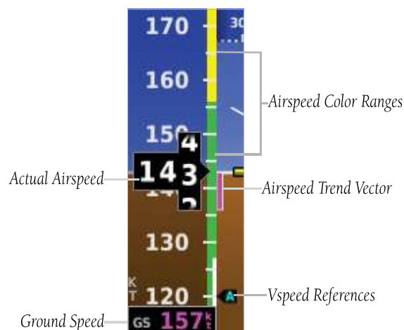
Figure 2-2 Airspeed Indicator
