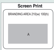
BOX222 Mace Gift Box E-flute board | 240(l) 150(w) 60(h)
