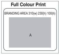
BOX221 Ljara Gift Box with handle E-flute board | 310(l) 230(w)100(h)
