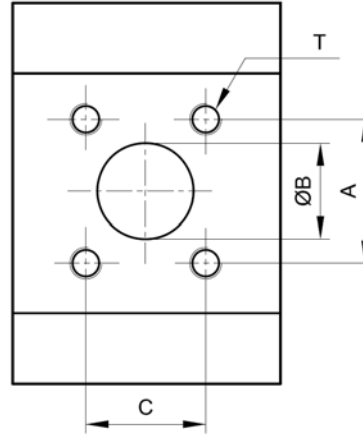
TİP 2 TYPE 2 KARE TİP PORT RECTANGULAR FLANGE
