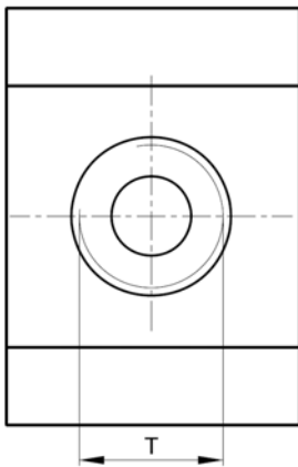
TİP 4 TYPE 4 UNF DİŞ ORİNG BOSLU UNF THREAD WITH ORING BOSS
