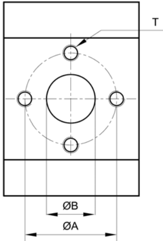
TİP 1 TYPE 1 KARE TİP PORT RECTANGULAR FLANGE
