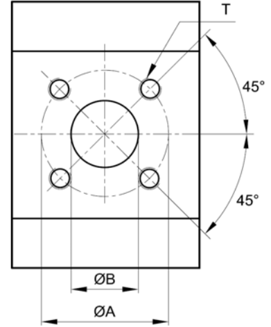
TİP 3 TYPE 3 KARE TİP PORT RECTANGULAR FLANGE
