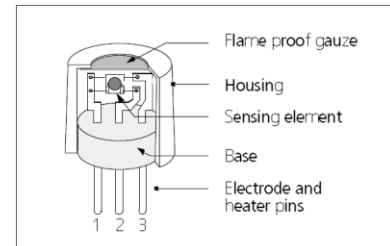
Fig2 .Structure
