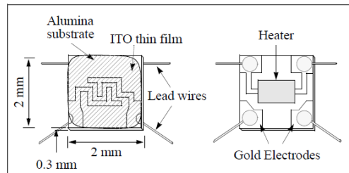
Fig 1. Sensing Elements
