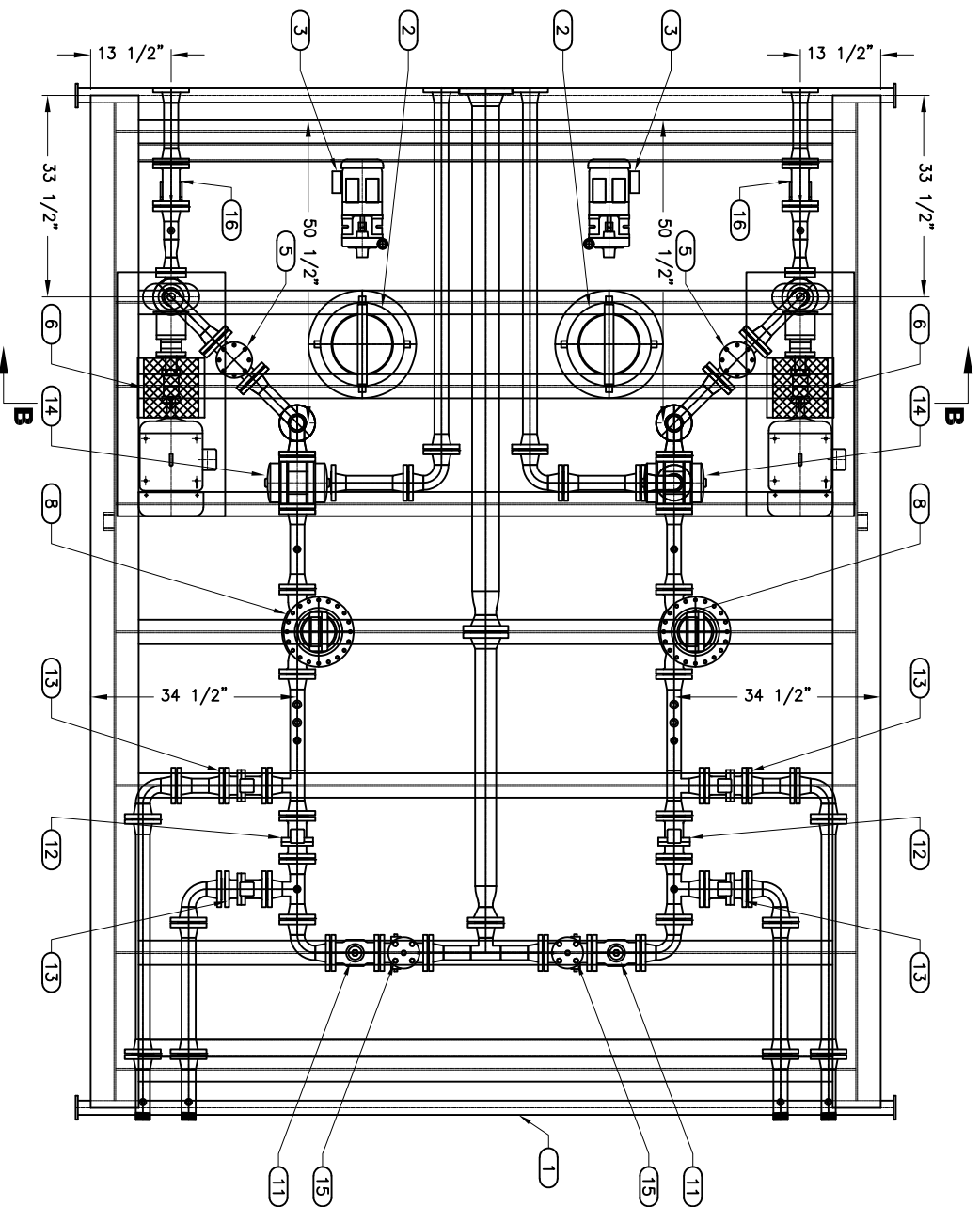
PLAN VIEW
