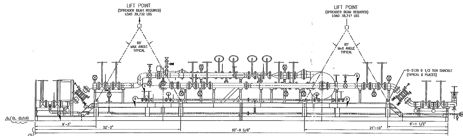
ELEVATION VIEW TOTAL LIFT WT = 78,480
