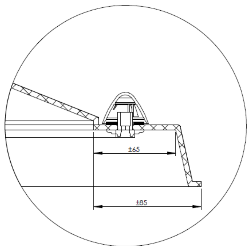
DETAIL B
